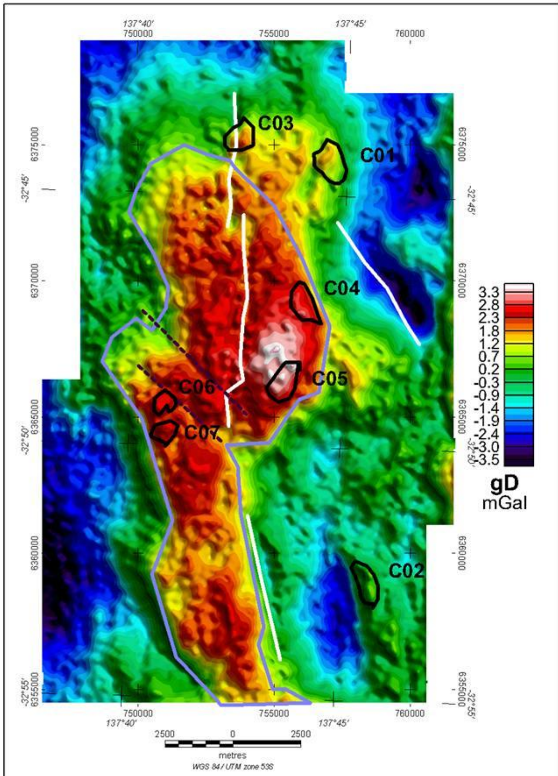
Fig 2 - Preliminary Targeting, gravity data
