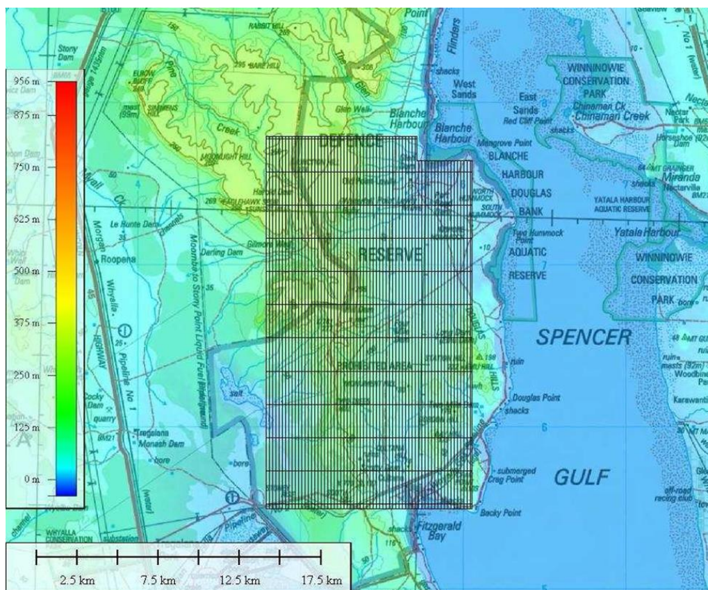
Fig 1 - HeliTEM flight lines
