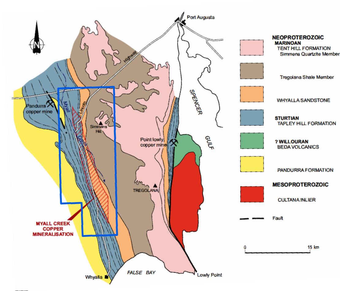
Figure 3: Myall Creek regional geology 1 with EL6140 in blue polygon
